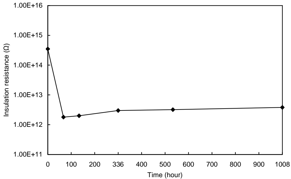
SIR GRAPH
