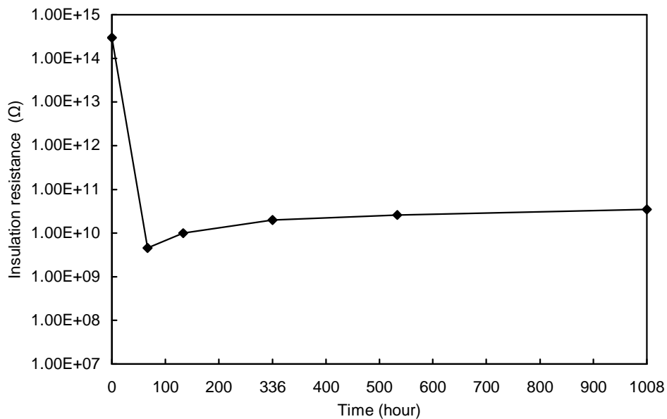
SIR GRAPH
